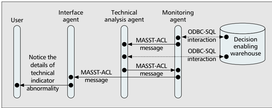
■ Figure 5. Agent interactions for monitoring technical indicator abnormality.
